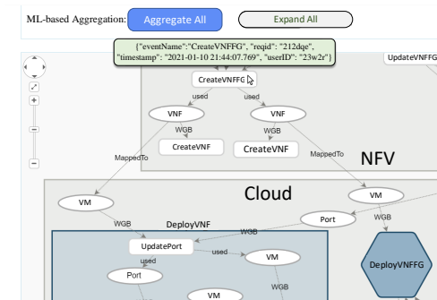
Fig. 22: Example screenshot of ProvTalk showing the aggregated and expanded cloud-level nodes and the information shown while hovering a node.
